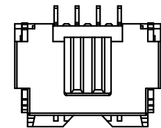
03P-05P Single Hole Scale 1:1
