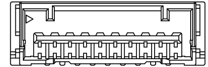
10 PIN
